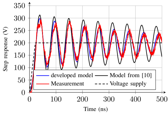
Fig. 8. Measured and simulated voltages at the input of the 56-turn winding.
