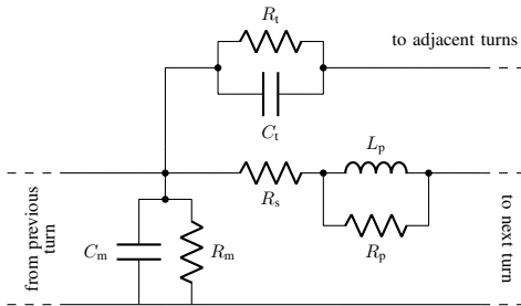
Fig. 2. Lumped parameter equivalent circuit of one turn.
