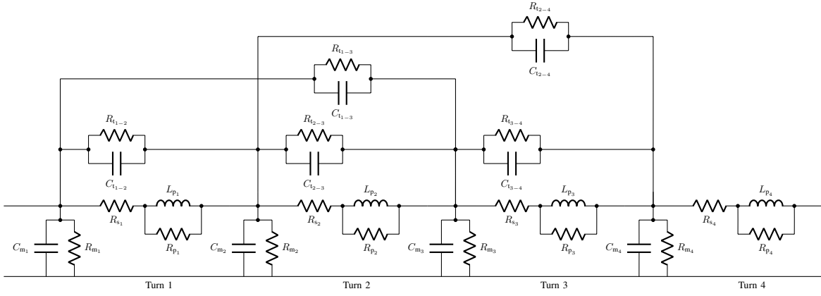
Fig. 1. Lumped parameter equivalent circuit of a 4-turn winding.
