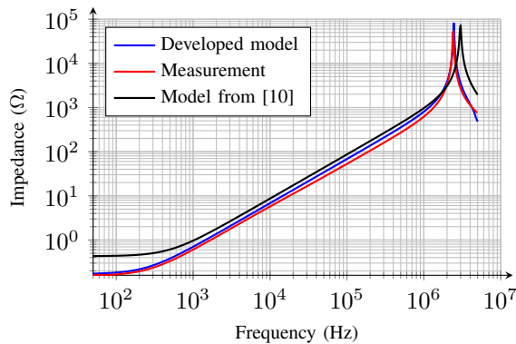
Fig. 9. Measured and simulated impedances of the 56-turn winding.
