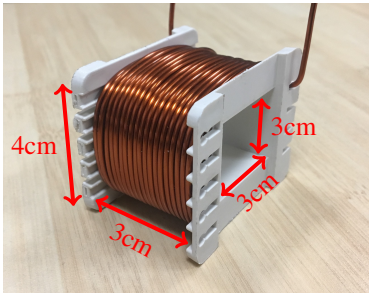
Fig. 4. 56-turn winding.
