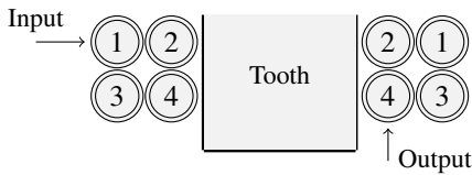
Fig. 3. An example of a 4-turn winding.
