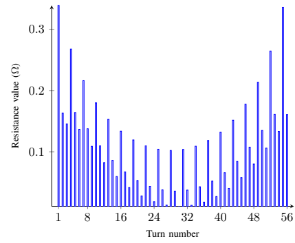
Fig. 5. Values of Joule losses resistances.
