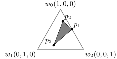
Figure 1: Example of extreme points p_1 , p_2 and p_3 using a barycentric representation.
