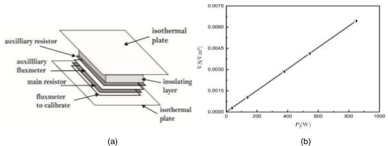
Figure 4- Schematic drawing of the used heat flux sensors: (a) Heat flux sensor's sketch (b) Calibration apparatus
